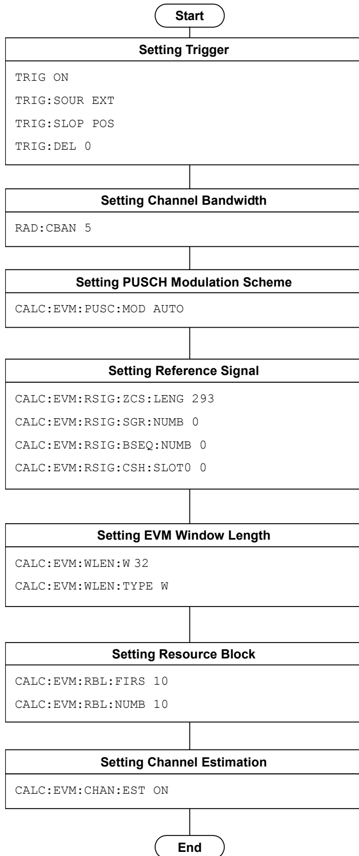
Figure 1.2.3-1 Flow of Common Settings for Modulation and Command Example
