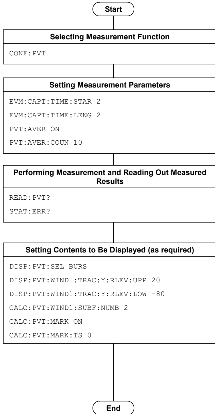
Figure 1.2.5-1 Flow of Power vs Time Measurement and Command Example
